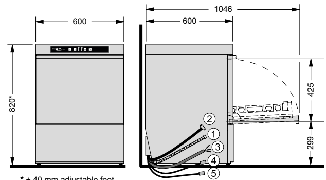
Undercounter dishwasher model F503
